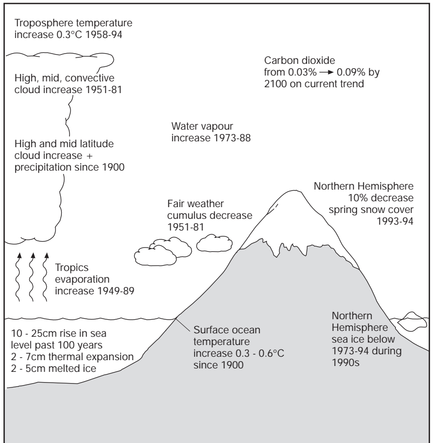
Figure 5: Identified changes in atmospheric and hydrological characteristics
